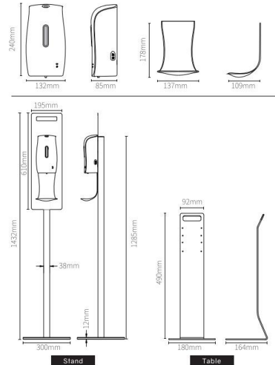
Unit Dimension
