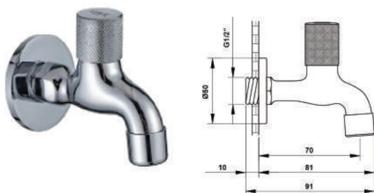
Single Bib Tap
