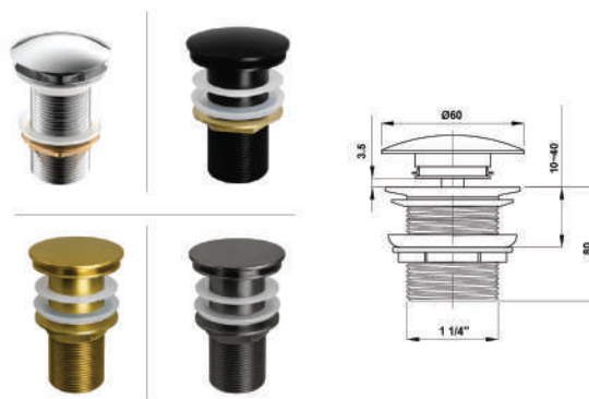
Push Waste (Brass)
