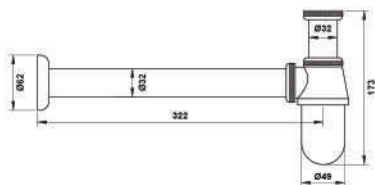
Bottle Trap EX024
