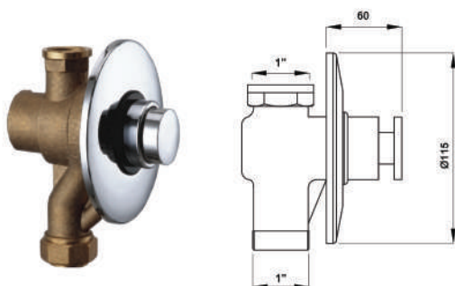
Toilet Flush Valve GS8016
