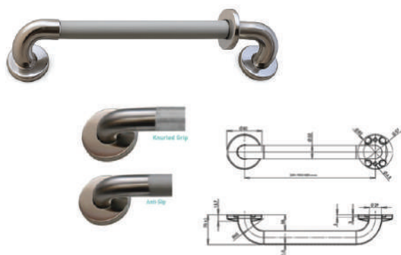
Handicap Grab Bar Straight ZHBS001, ZHBS002, ZHBS003
