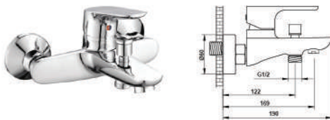
Bath Mixer ZTTN200
