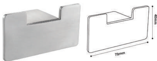
Stark Coat Hook
