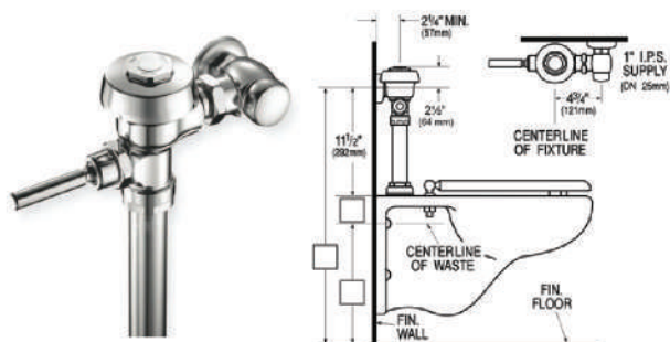
Toilet Flush Valve ZFV005
