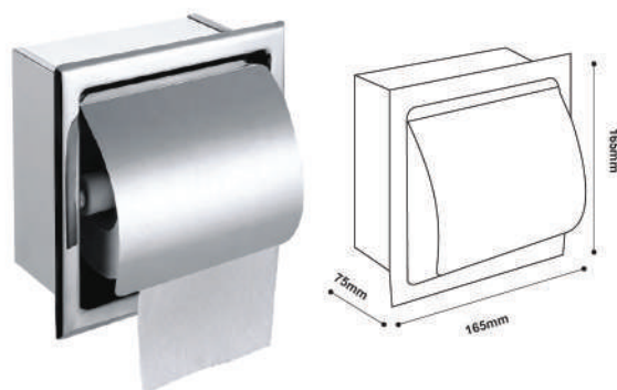
Concealed Paper Holder With Cover
