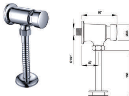
Urinal Flush Valve GS5210
