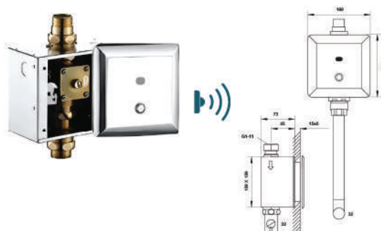
Sensor Toilet Flush Valve ZY1999
