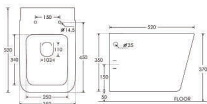
Wall Hung Toilet ZWHT101, ZWHT101MB
