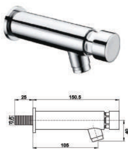
Self Closing Tap Wall Type
