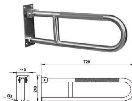
Handicap Flip-Up Grab Bar ZHBU01
