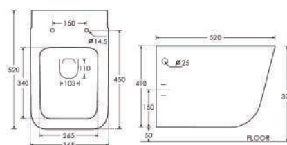
Wall Hung Toilet ZWHT102, ZWHT102MB
