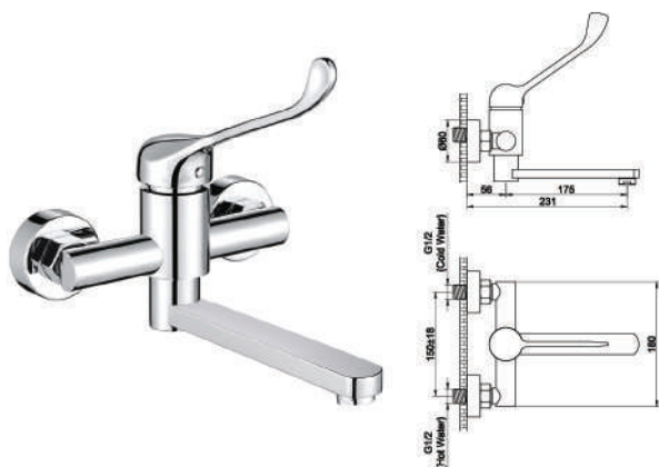
Elbow Action Faucet Wall Mounted UB001
