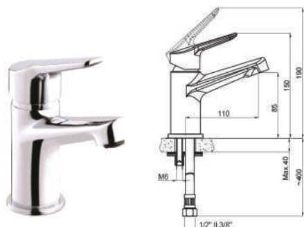
Normal Basin Mixer
