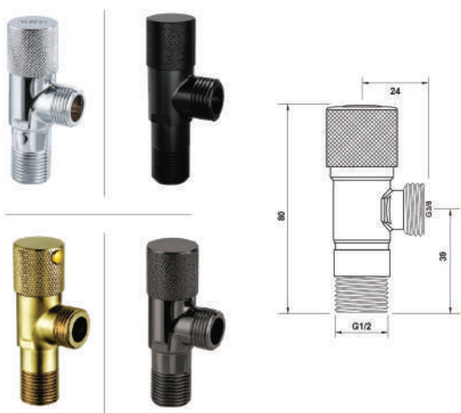
Angle Valve Full Turn
